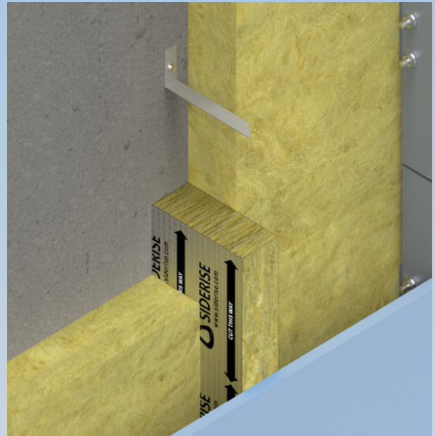
Siderise RV vertical cavity barrier
